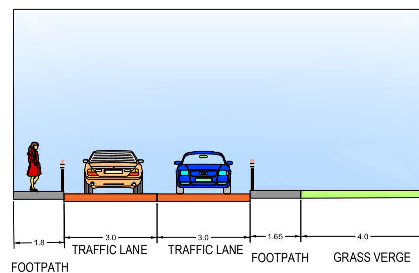
PROPOSED CROSS SECTION A-A
