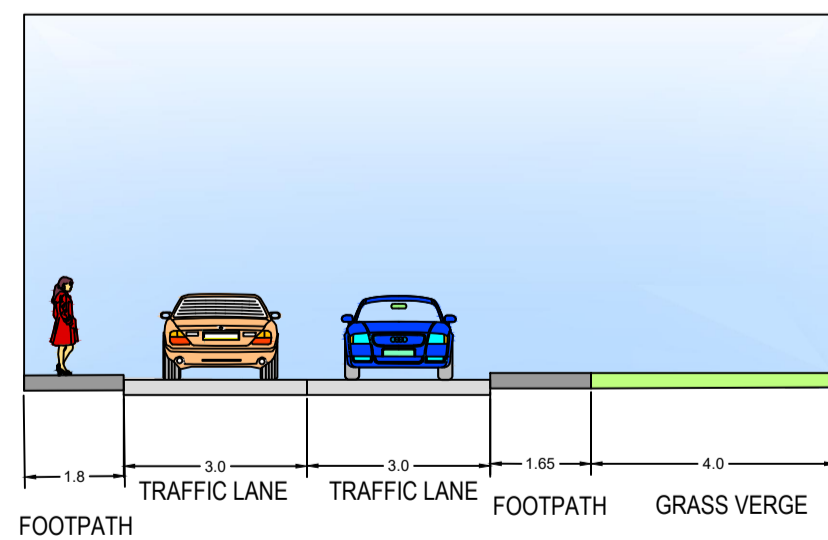
EXISTING CROSS SECTION A-A
